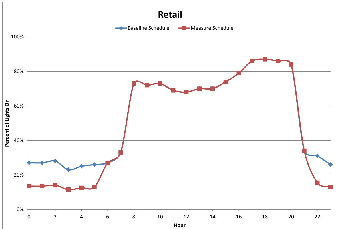
Figure 28 Retail schedule with shutoff controls
