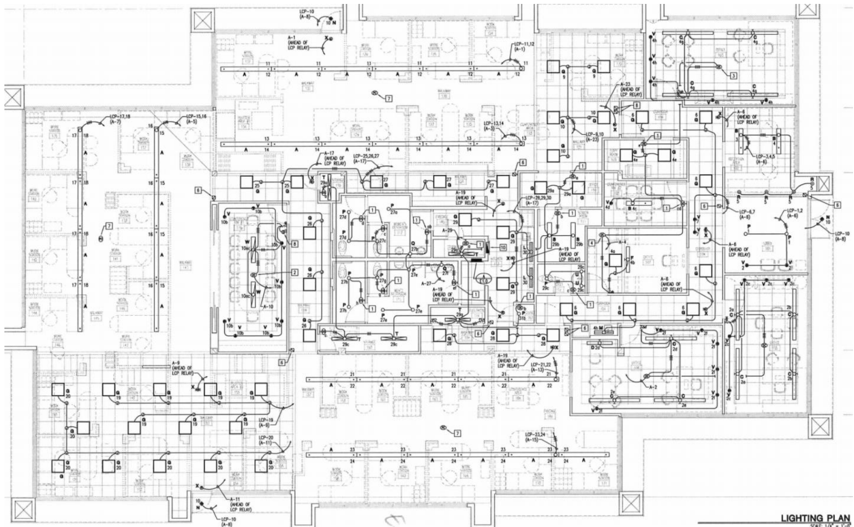
Figure 55 Small Office Prototype Reflected Ceiling and Floor Plan
