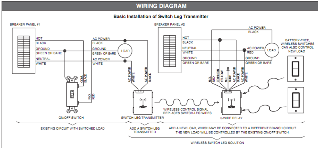
Figure 19 Wiring Diagram for Installation of a Wireless Switch Leg Transmitter
