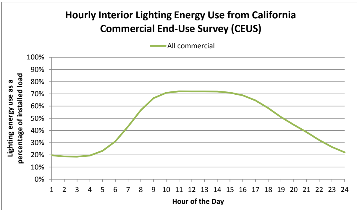
Figure 30 Hourly Interior Lighting Schedule from CEUS
