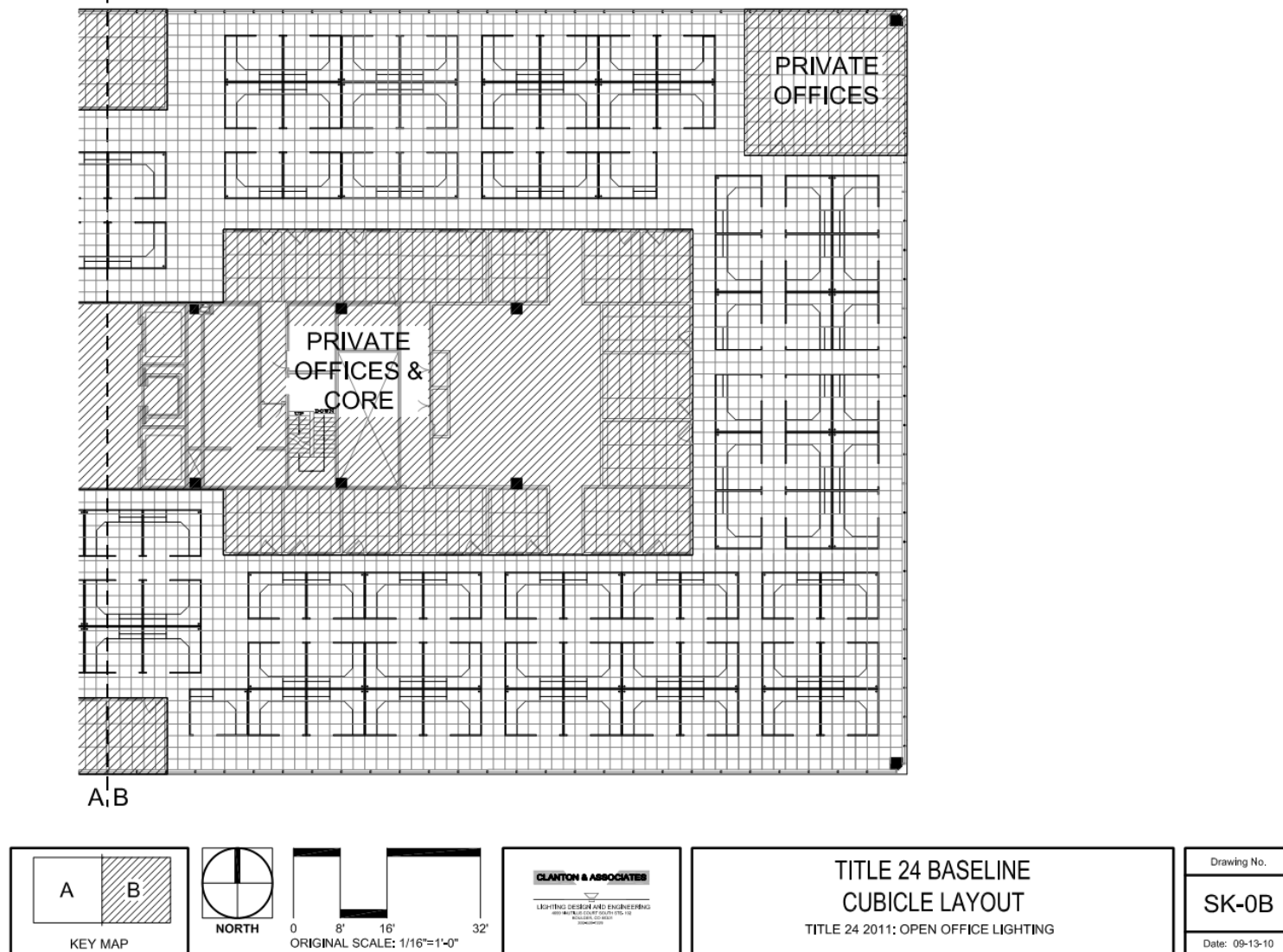
Figure 57 East Wing of Large Office Prototype Floor Plan
