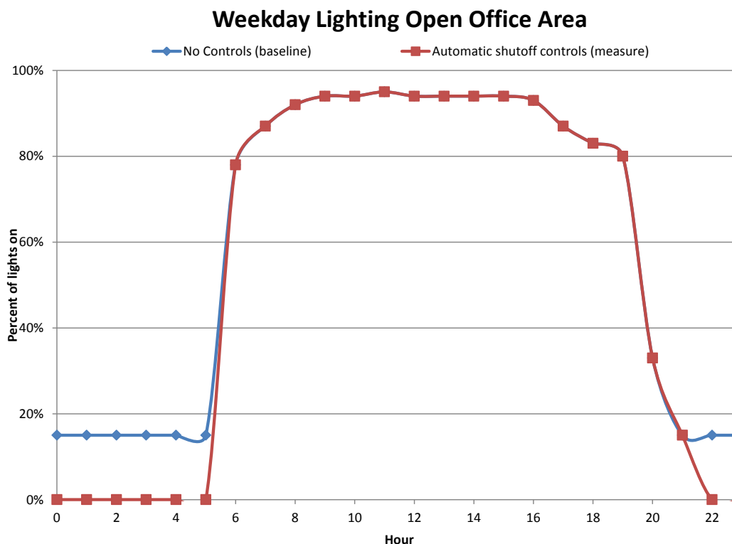
Figure 26 Open Office Area Weekday Lighting Schedule
