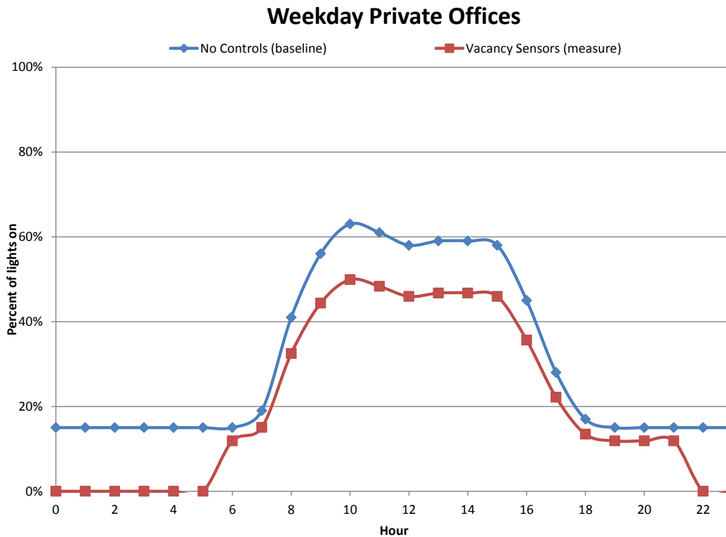
Figure 27 Private Office Weekday Lighting Schedule
