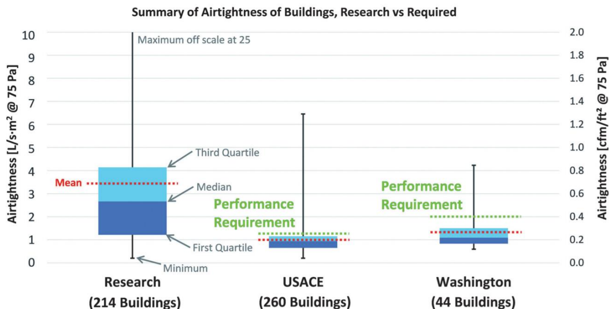
Figure 3: Distribution of airtightness performance of buildings tested for research purposes, and for compliance with United States Army Core of Engineers and Washington state airtightness requirements.
