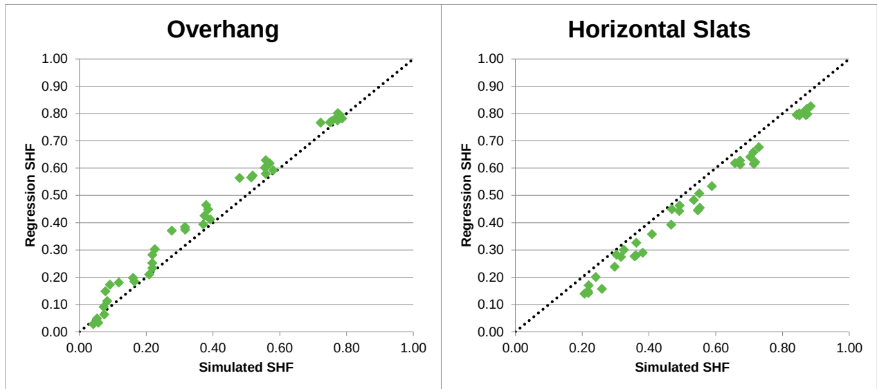
Figure 5: Shading factor regression curve versus simulated values.
